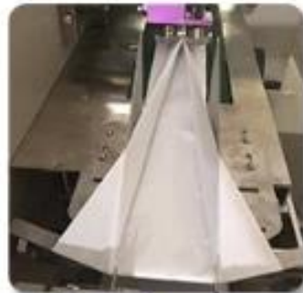
Bag former
